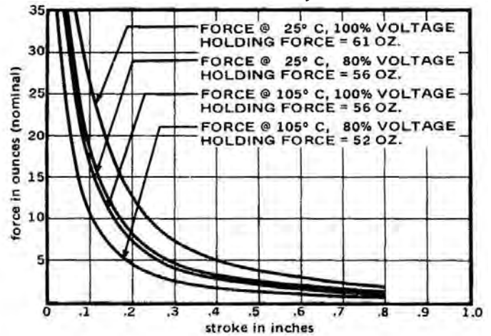
DC Continuous Duty - 8 Watts
