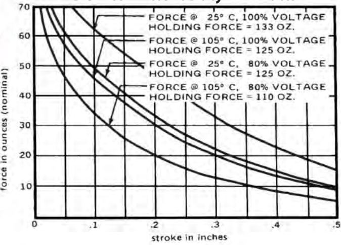
DC Pulse Duty - 85 Watts
