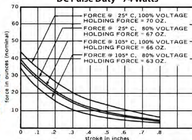
DC Pulse Duty - 74 Watts
