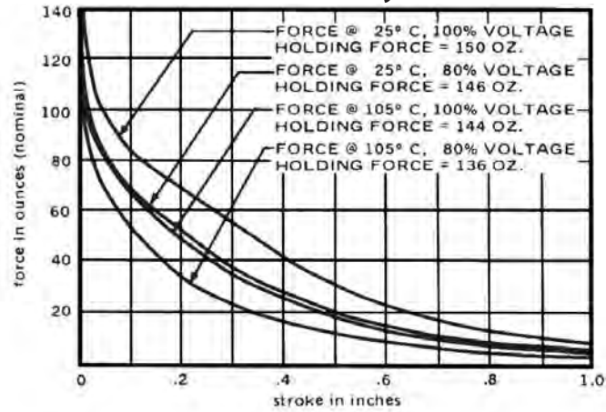
DC Continuous Duty - 13 Watts
