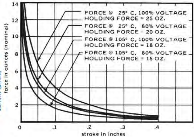
DC Intermittent Duty - 11 Watts
