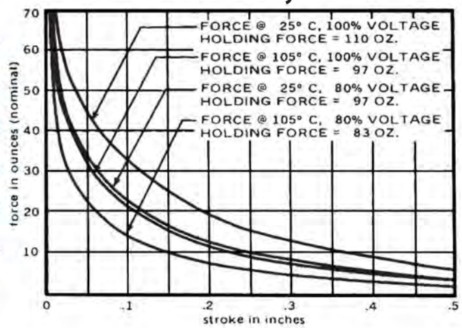
DC Intermittent Duty - 21 Watts
