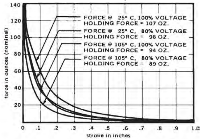
DC Continuous Duty - 11 Watts
