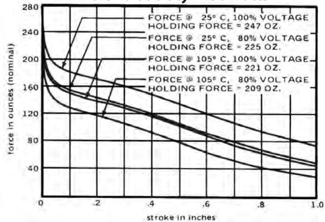
DC Pulse Duty - 130 Watts
