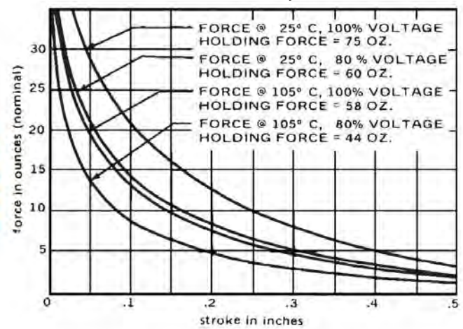
DC Continuous Duty - 8.6 Watts
