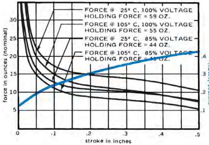
AC Continuous Duty - 13.7 VA
