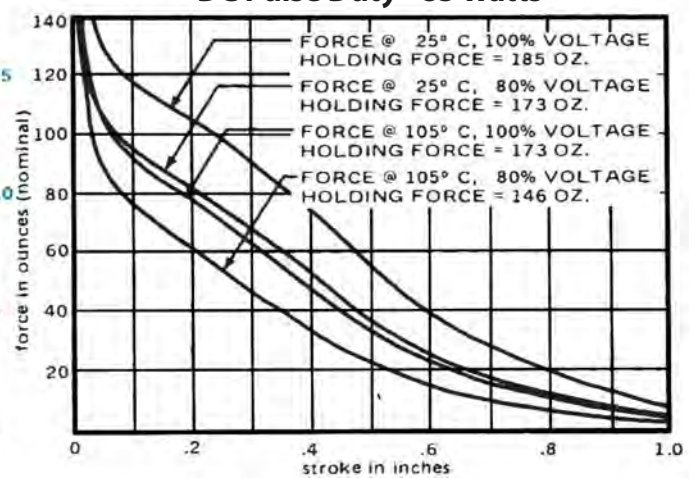
DC Pulse Duty - 85 Watts
