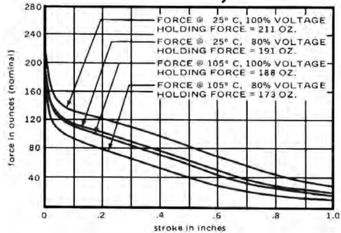
DC Intermittent Duty - 48 Watts
