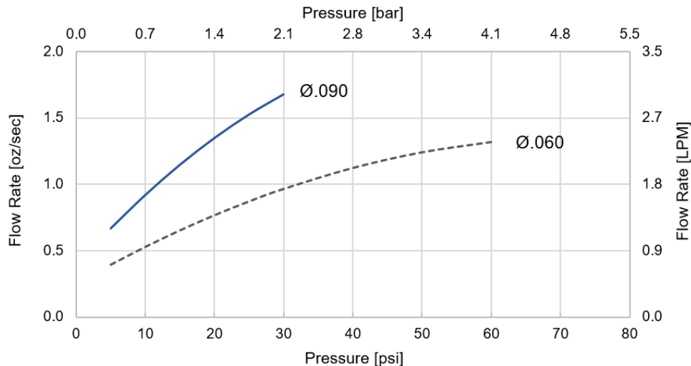
DSV28 Flow Curves Dry Plunger - Water
